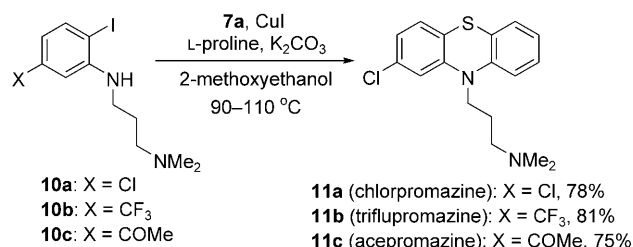
Scheme 1. Synthesis of three psychotropic promazine drugs.
